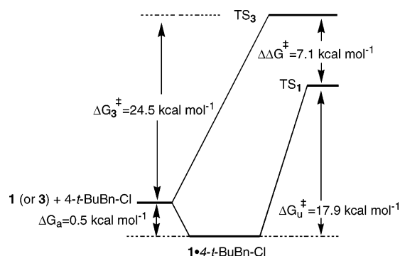
FIGURE 3. Reaction coordinate diagram for the reaction of 4- t -BuBnCl with macrocycle \mathbf{1} or control amine \mathbf{3} .
